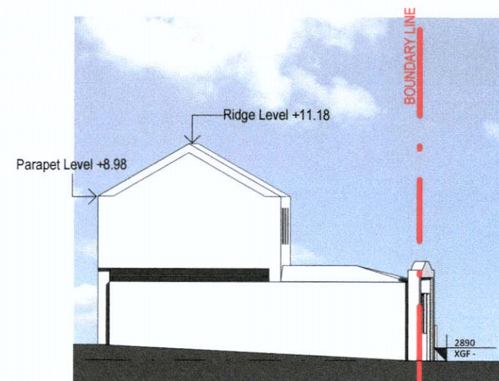
③ Elevation CC 1 : 200
