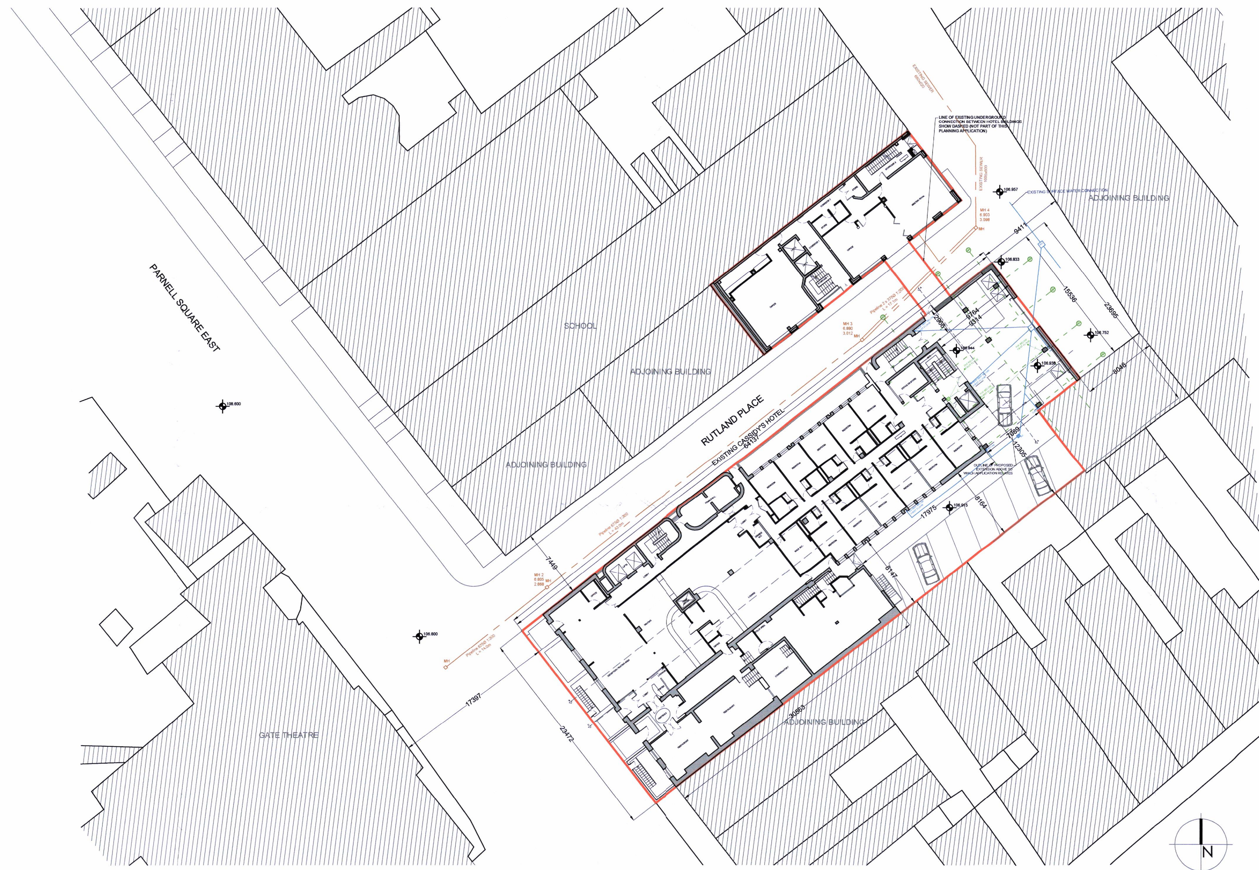
SITE MAP SCALE 1:250 AREA & SCHEDULE Area of site 1.78 Ha Area of new building proposed within the site 833 sq.m Area of existing building to be demolished None
