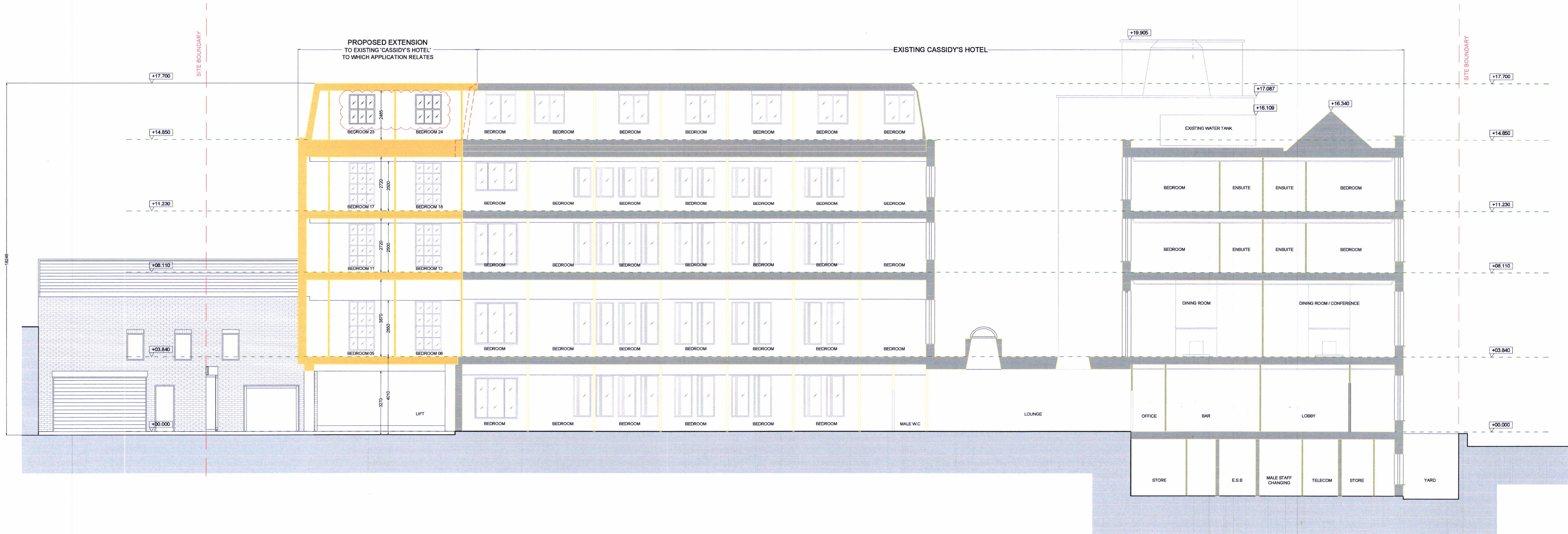
SECTION C-C SCALE 1:100
