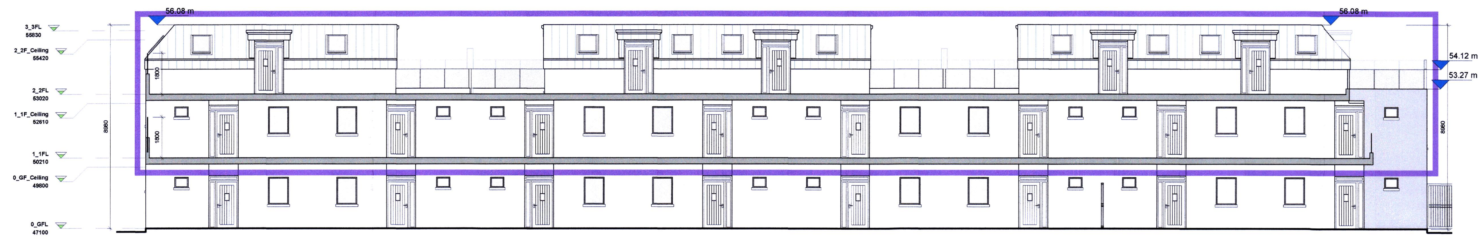
East Courtyard Elevation (SN Section) 1 : 100
